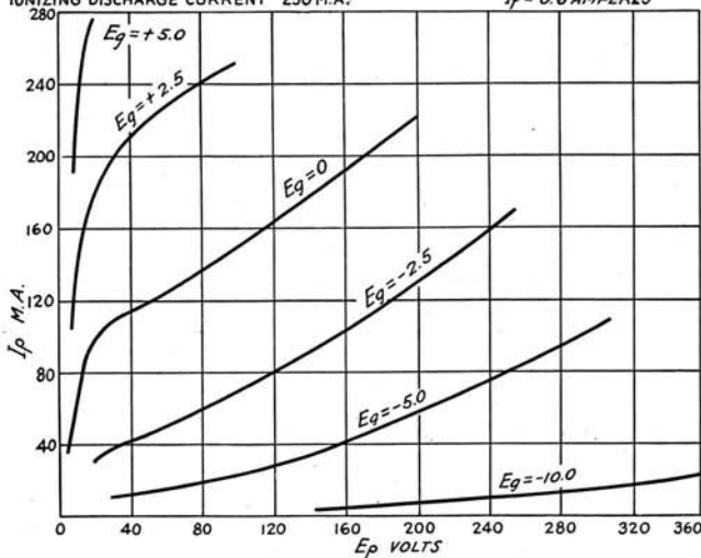
FIG. 5 RK-100 PLATE CHARACTERISTICS - IONIZING DISCHARGE CURRENT 250 M.A.
