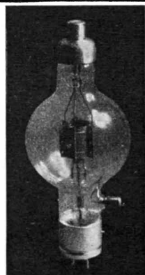
EIMAC 50-T
