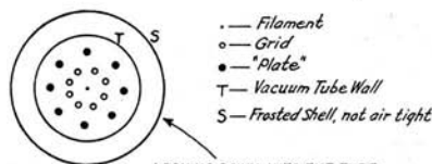
LOOKING DOWN INTO THE TUBE CONSTRUCTION AND CONNECTION OF D-21 TUBE
