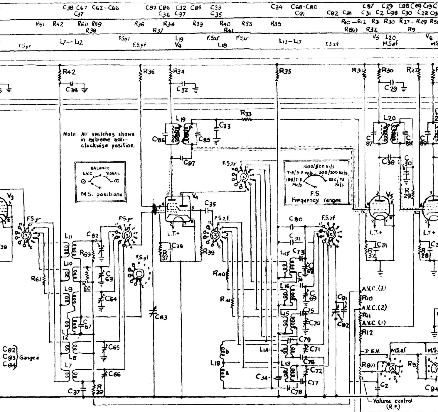
R.1155 AND R.1155D CIRCUIT DIAGRAM INCLUDING R.1155A, R.1155E, AND R.1155M MODIFICATIONS
