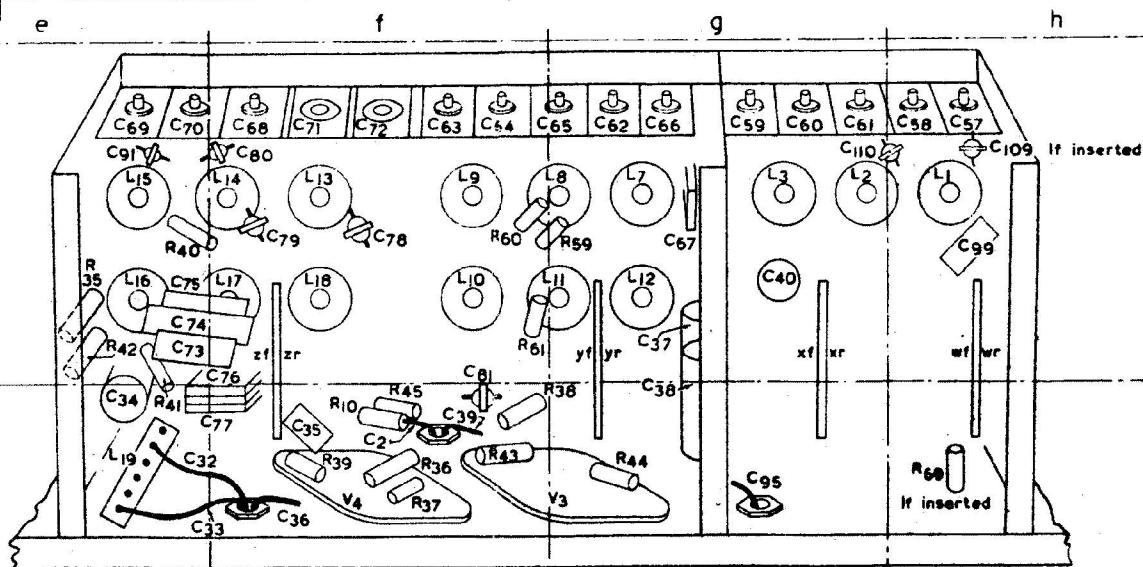
INSIDE VIEW OF RANGE CONTAINER
