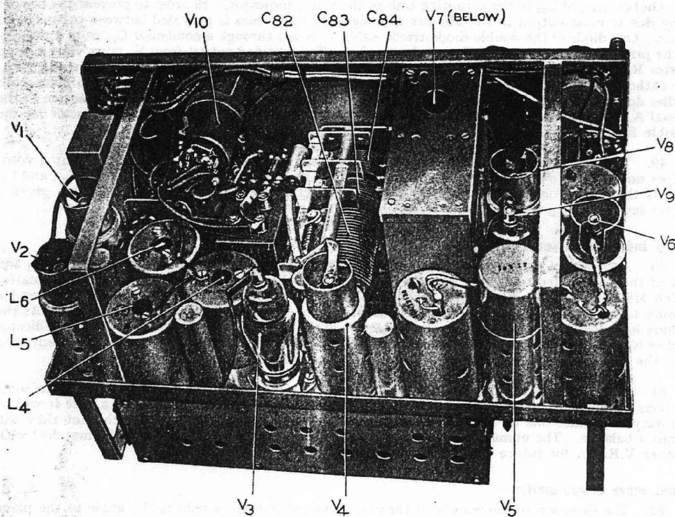
FIG. 15.—R.1155 CHASSIS, UPPER DECK
