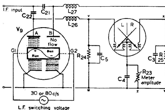
FIG. 13.—SIMPLIFIED VISUAL INDICATOR SWITCHING CIRCUIT
