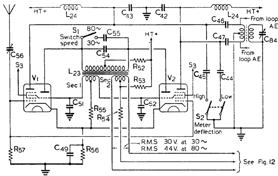
FIG. 11.—L.F. OSCILLATOR SWITCHING CIRCUIT
