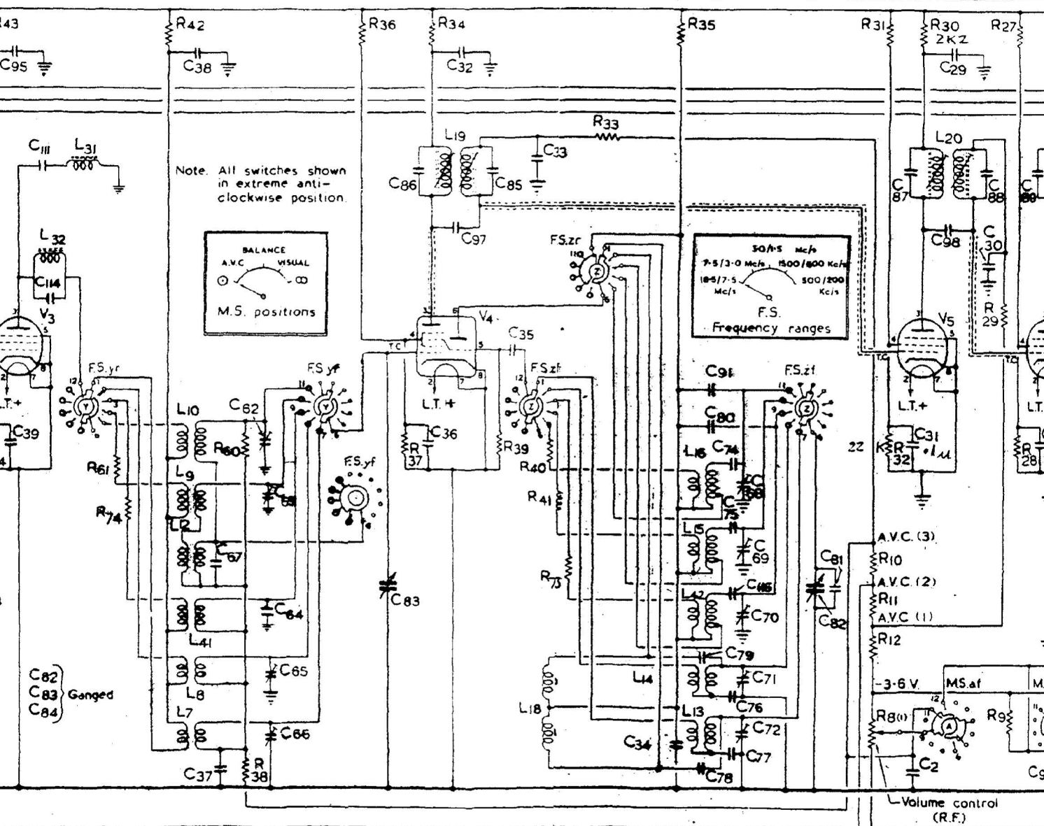
R 1155 L AND R 1155 N CIRCUIT DIAGRAM
