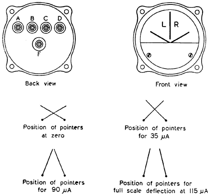
FIG. 25.—VISUAL INDICATOR, TYPE 1
