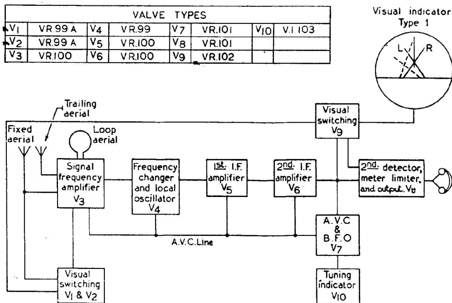
FIG. 2.—SCHEMATIC DIAGRAM
