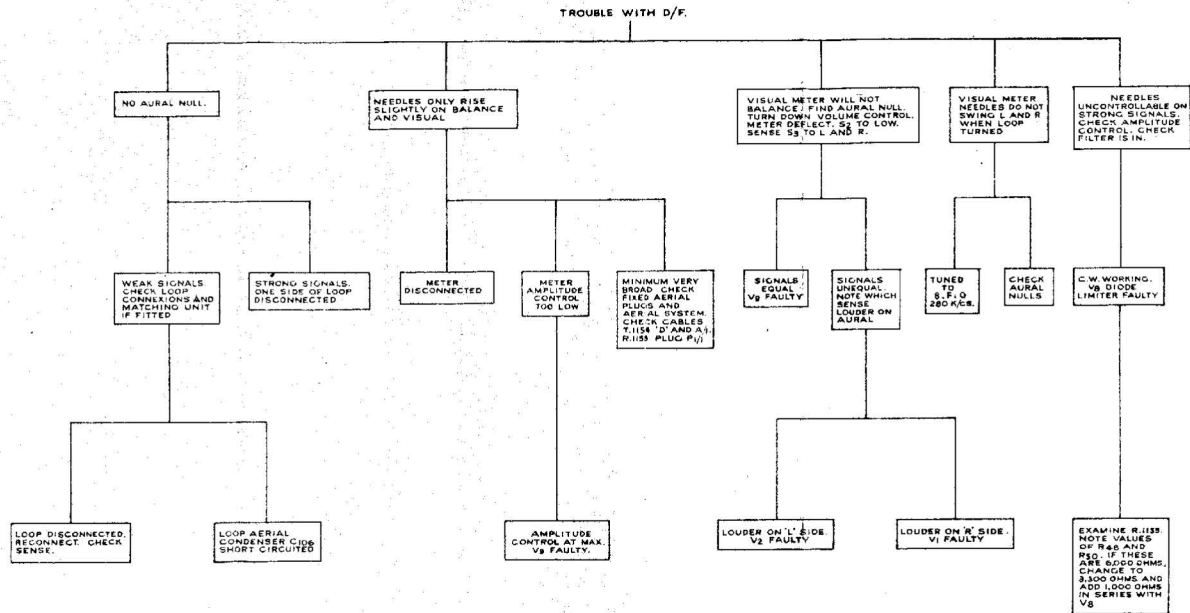
D. F. SWITCHING CIRCUITS — TROUBLE LOCATION CHART
