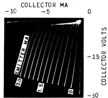
Fig. 12 - Oscillogram of output characteristic of RCA developmental point-contact transistor.
