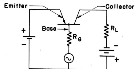
Fig. 19 - Transistor grounded-emitter amplifier circuit.
