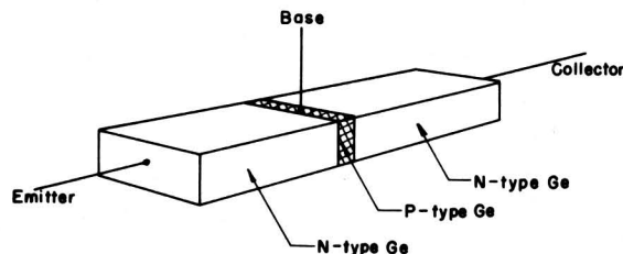
Fig. 15 - Arrangement of "n" and "p" layers in germanium crystal of n-p-n junction transistor.
