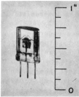
Fig. 6 - RCA developmental point-contact transistor.
