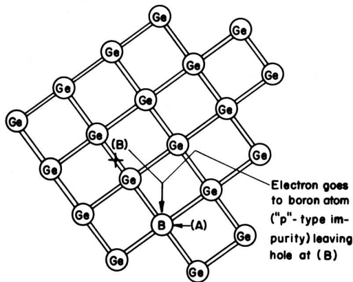
Fig. 5 - Effect of p-type impurities on germanium conductivity.
