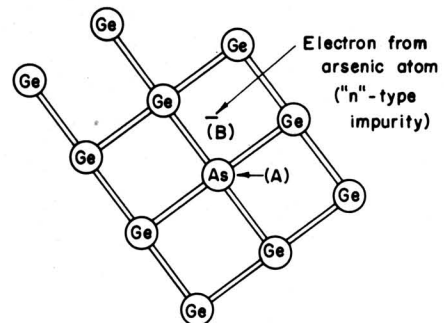
Fig. 4 - Effect of n-type impurities on germanium conductivity.
