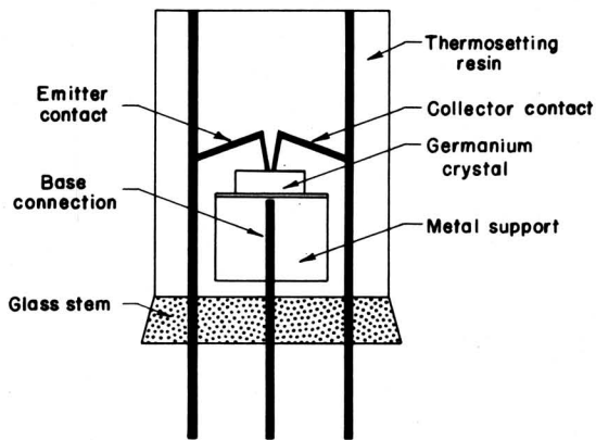
Fig. 7 - Construction of RCA developmental point-contact transistor.
