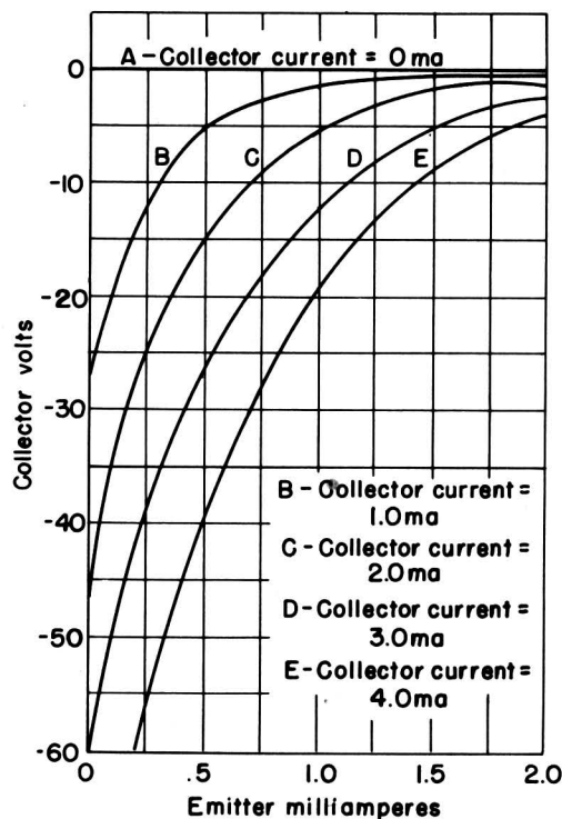
Fig. 14 - Transfer characteristic of RCA developmental point-contact transistor.
