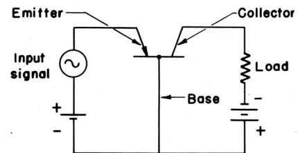
Fig. 8 - Transistor amplifier circuit.
