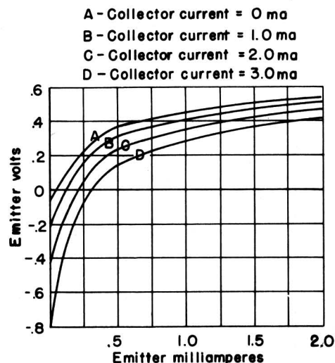
Fig. 9 - Input characteristic of RCA developmental point-contact transistor.
