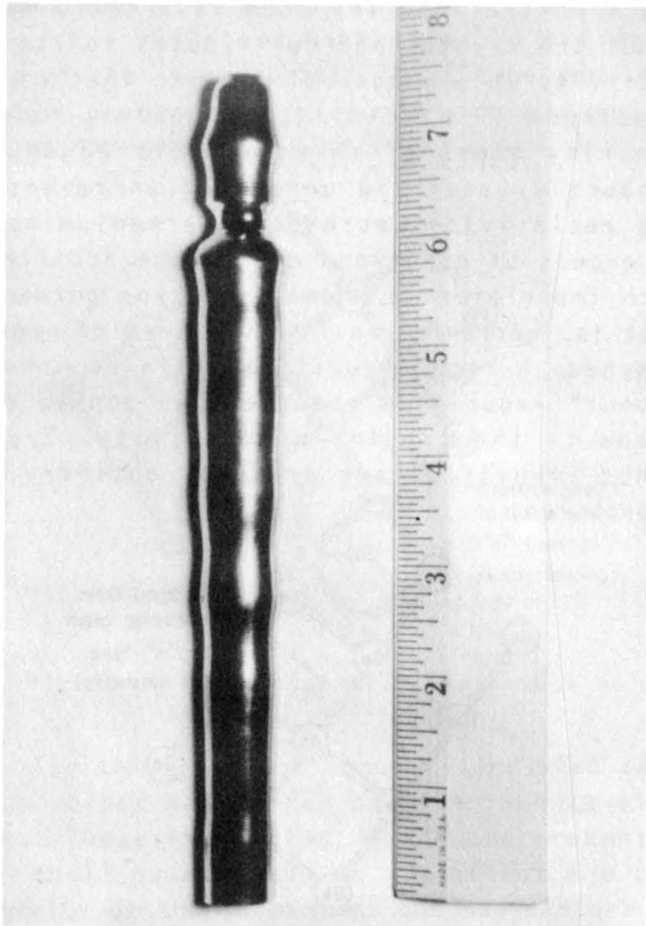
Fig. 2 - Single germanium crystal grown in crystal-growing apparatus shown in Fig. 1.
