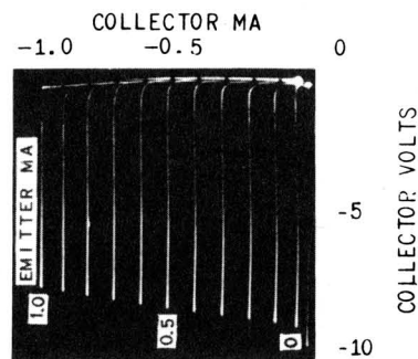
Fig. 17 - Oscillogram of output characteristic of RCA developmental p-n-p junction transistor.
