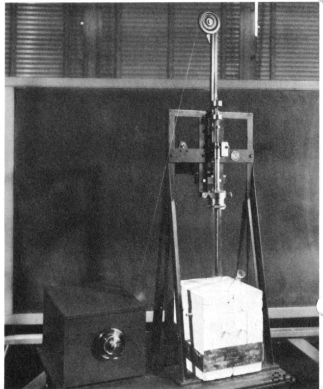
Fig. 1 - Apparatus for growing single germanium crystals.
