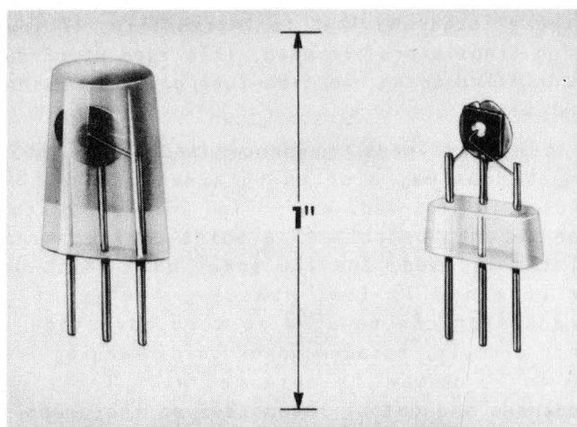
Fig. 16 - RCA developmental p-n-p junction transistor with and without plastic covering.
