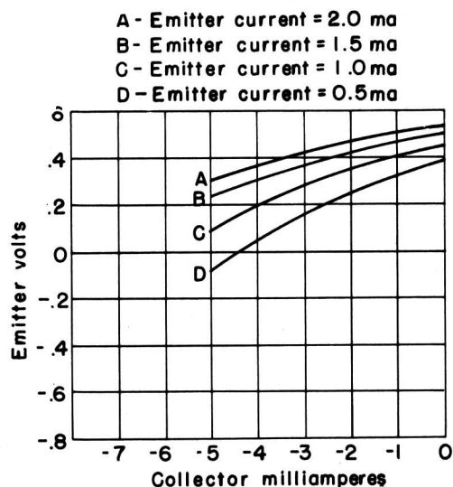
Fig. 10 - Feedback characteristic of RCA developmental point-contact transistor.
