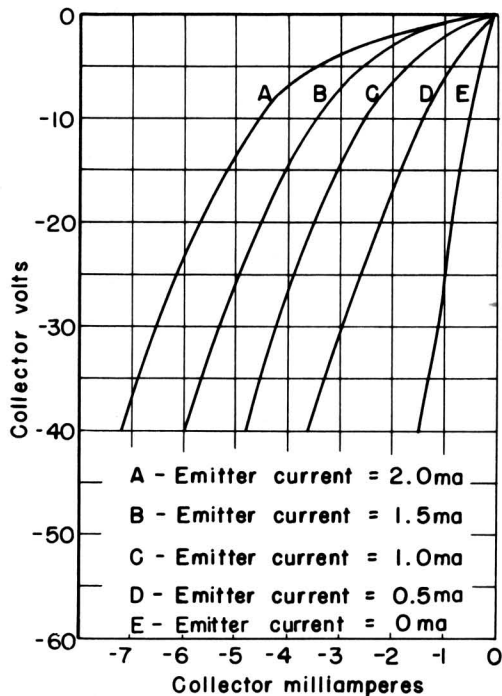
Fig. 11 - Output characteristic of RCA developmental point-contact transistor.
