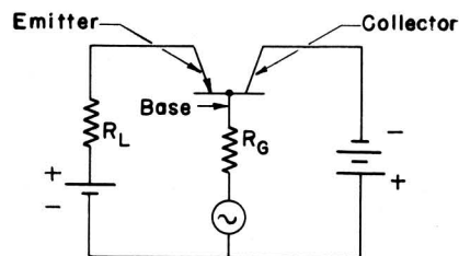
Fig. 20 - Transistor grounded-collector amplifier circuit.
