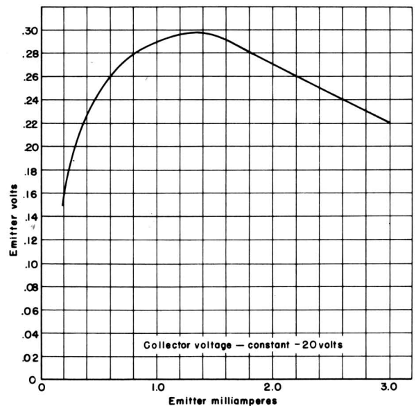
Fig. 13 - Negative input-resistance characteristic of RCA developmental point-contact transistor.
