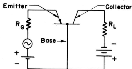
Fig. 18 - Transistor grounded-base amplifier circuit.
