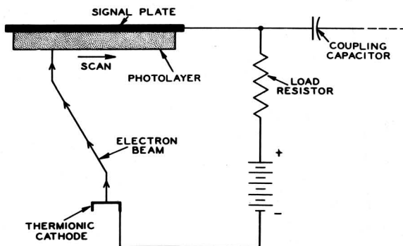
Fig. 1 - Basic principles of Vidicon operation.
