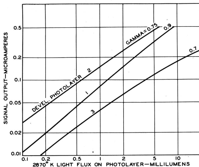
Fig. 5 - Transfer characteristics.
