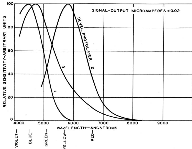
Fig. 6 - Spectral sensitivity characteristics.
