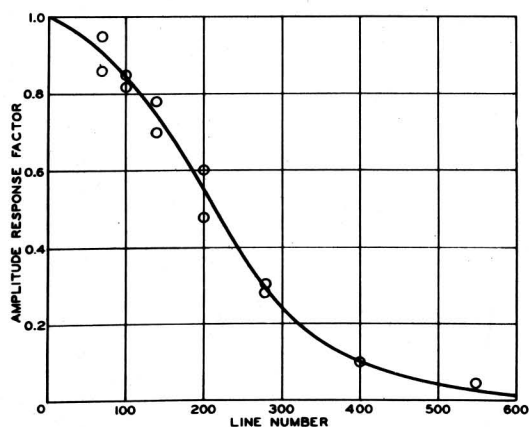
Fig. 4 - Amplitude response factor of typical developmental Vidicon.
