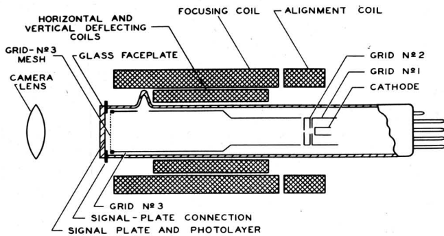
Fig. 2 - Arrangement of parts in Vidicon and positioning of associated components.
